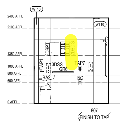
RACF STANDARD ROOM ENSUITE - ELEVATION 4 ELEVATION 4 Scale 1 : 50
