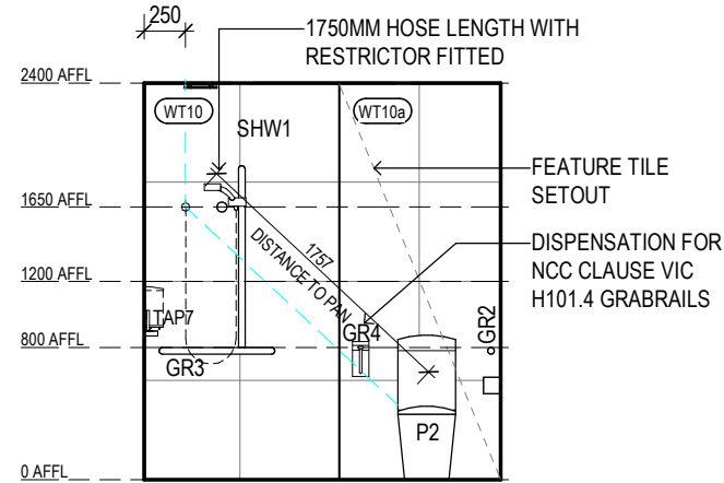
RACF STANDARD ROOM ENSUITE - ELEVATION 3 ELEVATION 3 Scale 1 : 50
