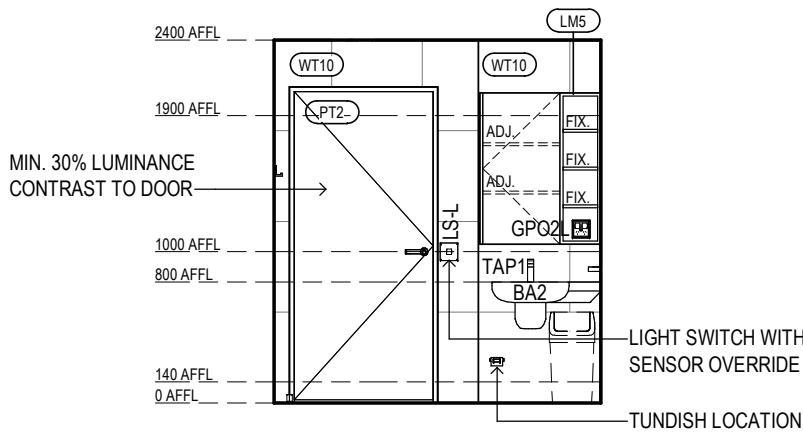
RACF STANDARD ROOM ENSUITE ELEVATION 1 Scale 1 : 50
