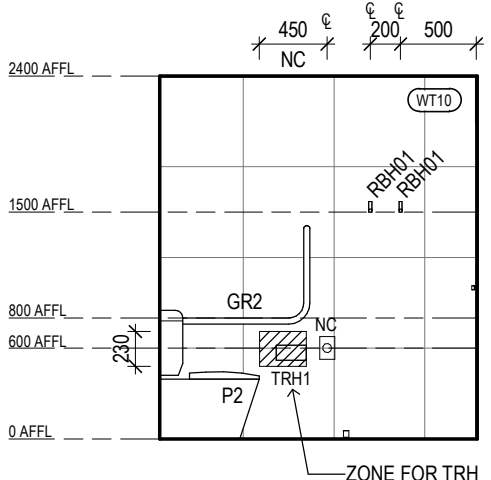
RACF STANDARD ROOM ENSUITE ELEVATION 2 Scale 1 : 50
